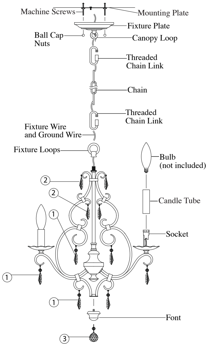
FIG: 1 CHAIN HUNG INSTALLATION
